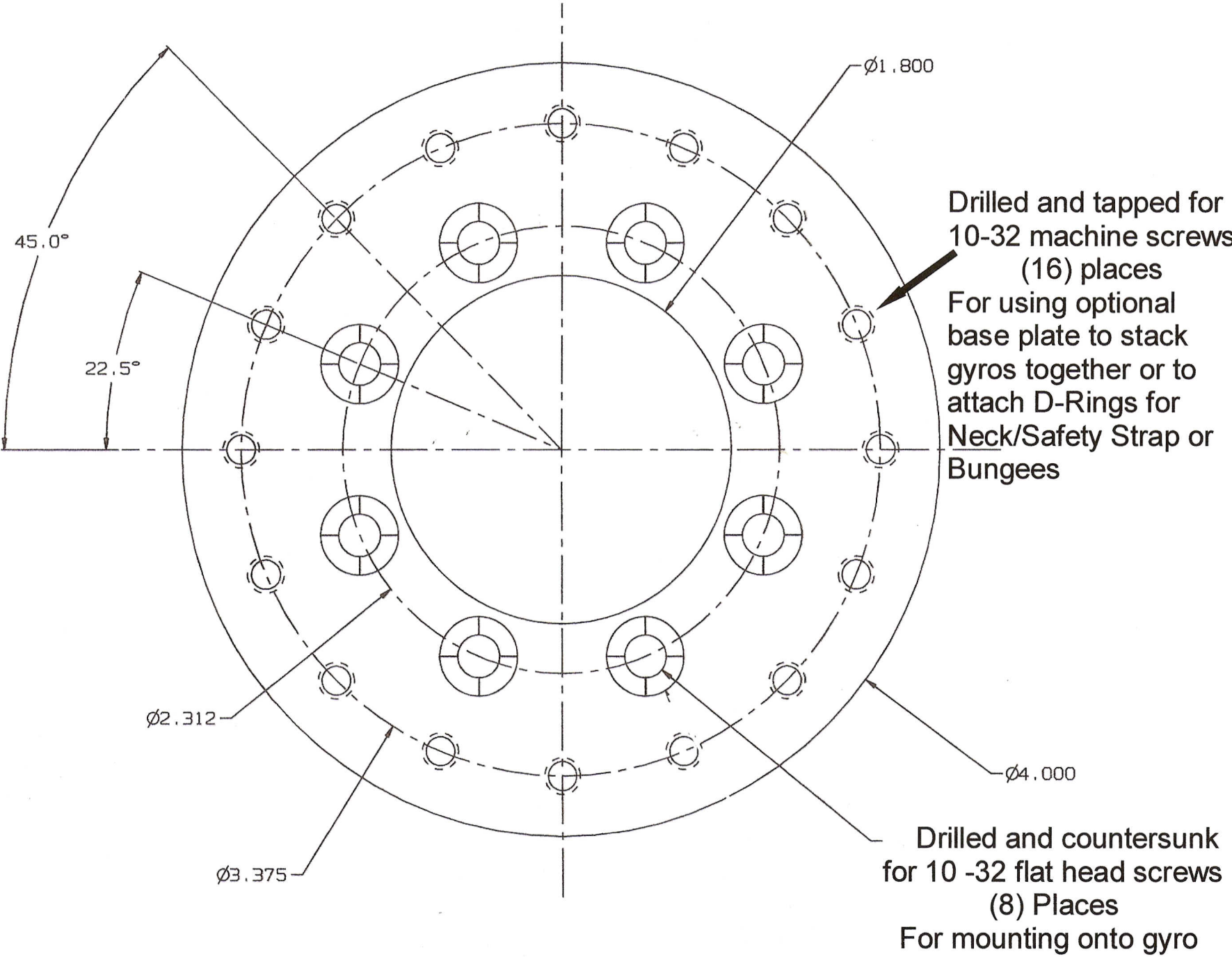
KS- 4x4 Optional Mounting Plate
